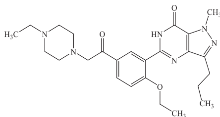
acetildenafile
