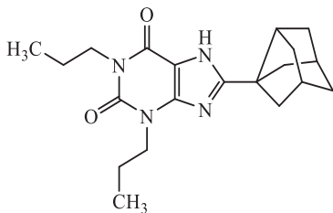
rolofylin
