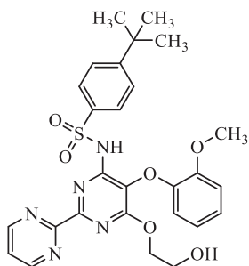
bosentan
