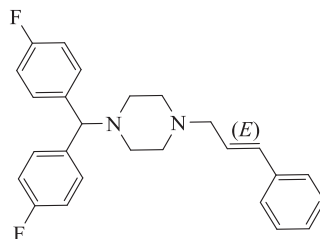
flunarizin
