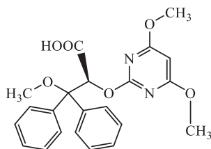
darusentan
